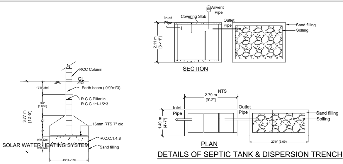
FOUNDATION DETAILS
