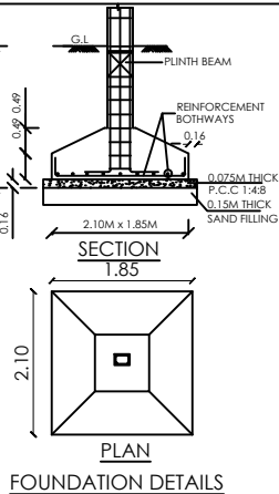
FOUNDATION DETAILS
