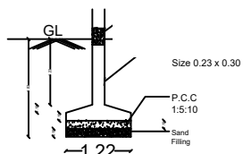
FOUNDATION DETAILS
