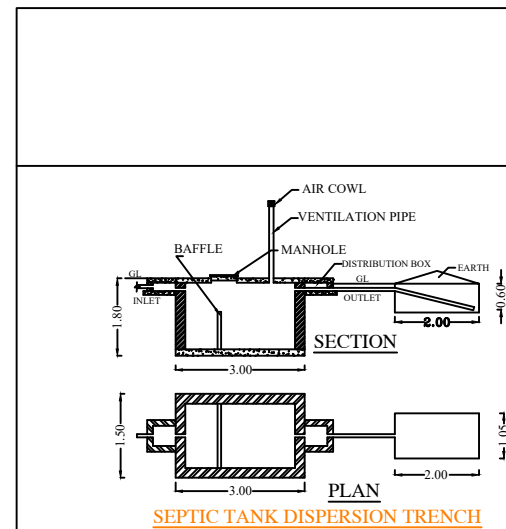
SEPTIC TANK DISPERSION TRENCH
