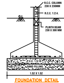
FOUNDATION DETAIL
