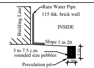
RAIN WATER HARVESTING PERCOLATION PIT
