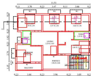
PRO. FIRST FLOOR PLAN
