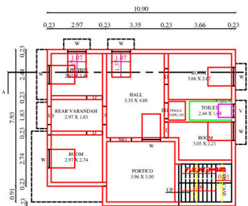
EX. GROUND FLOOR PLAN
