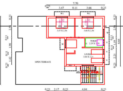
PRO. SECOND FLOOR PLAN
