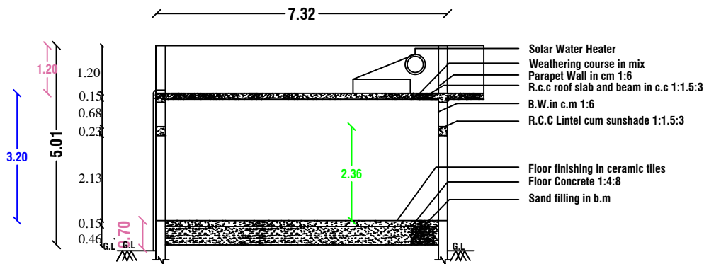
SECTION - "AB "
