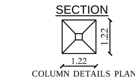
COLUMN DETAILS PLAN
