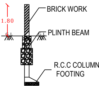
SECTION
