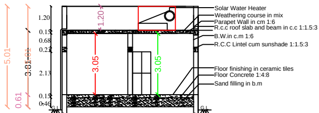
SECTION - "AB "
