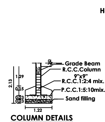
COLUMN DETAILS
