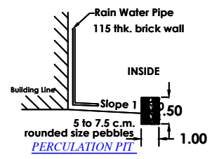
PERCOLATION PIT
