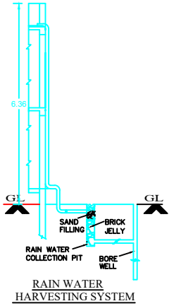
PERCOLATION PIT
