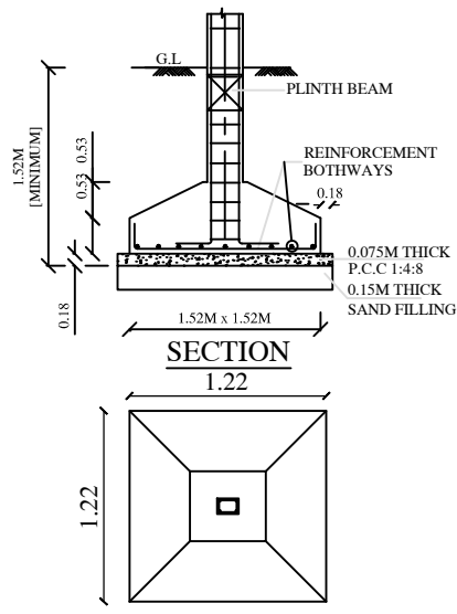
FOUNDATION DETAILS
