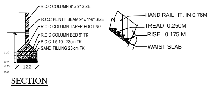
SECTION
