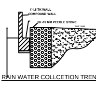
RAIN WATER COLLECTION TRENCH
