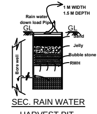
SEC. RAIN WATER HARVEST PIT
