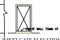
WICKET GATE ELEVATION
