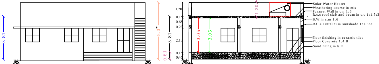
SECTION - "AB "
