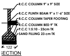
SECTION
