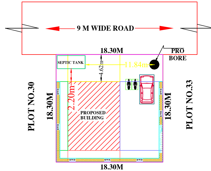
SITE PLAN
