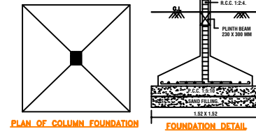
PLAN OF COLUMN FOUNDATION
