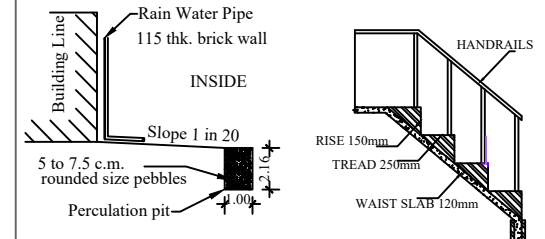
RAIN WATER HARVESTING PERCOLATION PIT
