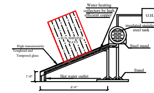
SECTION SOLAR WATER HEATER
