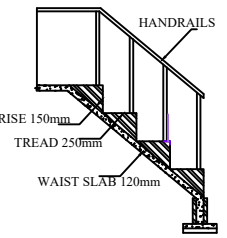
STAIRCASE DETAILS
