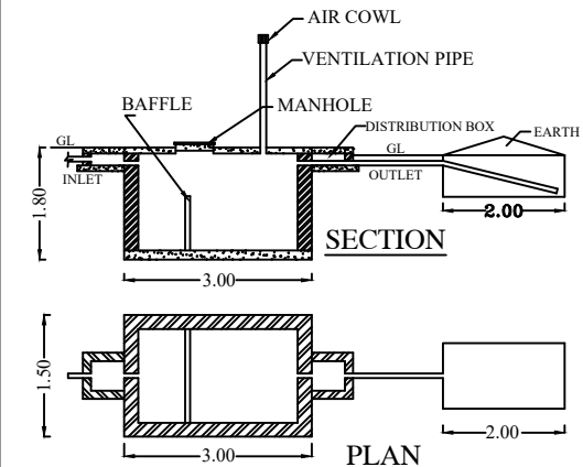
SEPTIC TANK DISPERSION TRENCH
