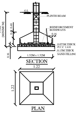
FOUNDATION DETAILS
