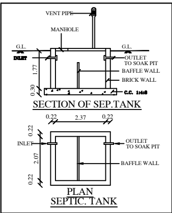
SECTION OF SEPTIC TANK
