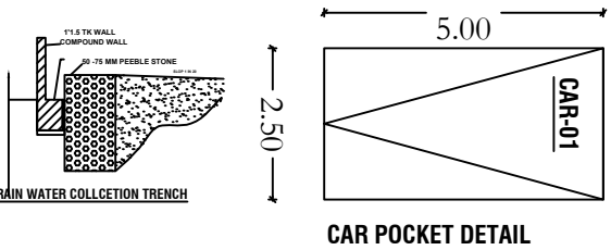
CAR POCKET DETAIL
