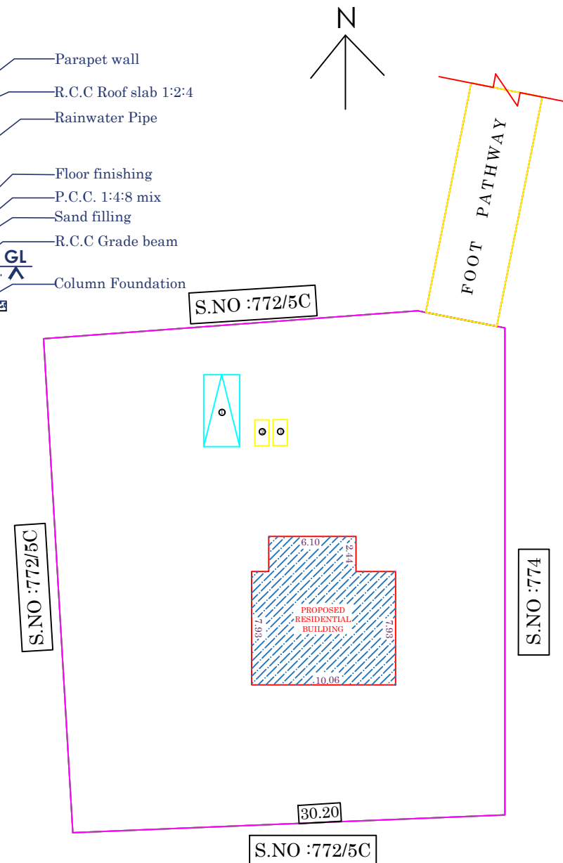
SITE PLAN
