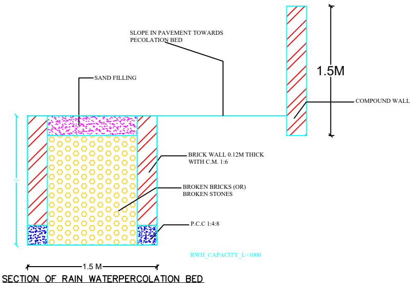
SECTION OF RAIN WATER PERCUATION BED
