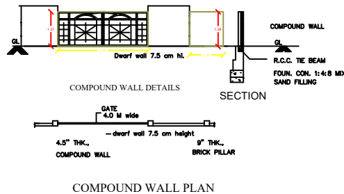
COMPOUND WALL PLAN
