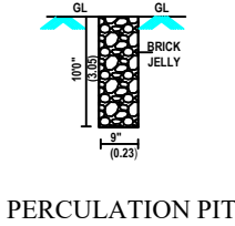
PERCUATION PIT
