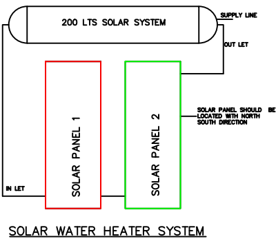
SOLAR WATER HEATER SYSTEM
