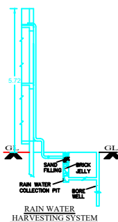
RAIN WATER HARVESTING SYSTEM
