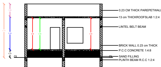
SECTION ON A - B
