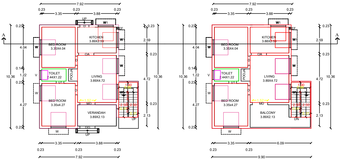
PRO.FIRST FLOOR PLAN
