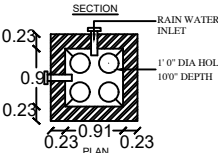
SECTION RAIN WATER HARVESTING PIT COLLECTING NOT TO SCALE
