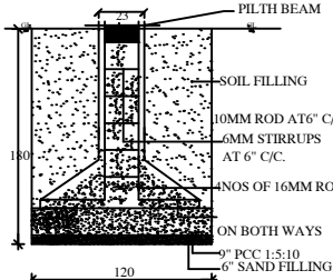
COLUMN FOOTING DETAIL NOT TO SCALE
