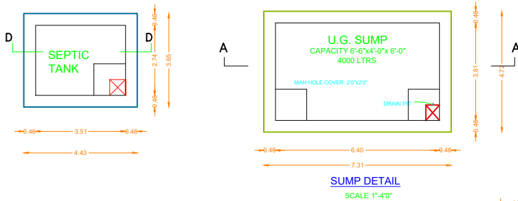
SCALE 1"=4'0"
