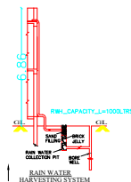
RAIN WATER HARVESTING SYSTEM
