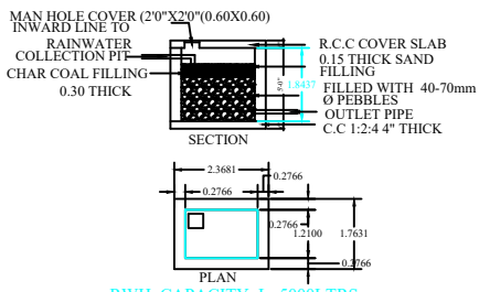
RWH CAPACITY: 1=5000LTRS DETAILS OF COLLECTION SUMP FOR RAIN WATER HARVESTING OF ROOF TOP RAIN WATER
