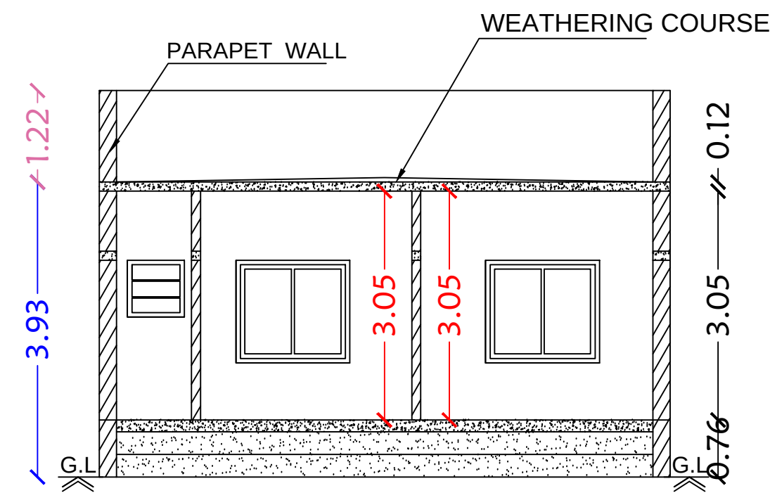
Section on-"AA"
