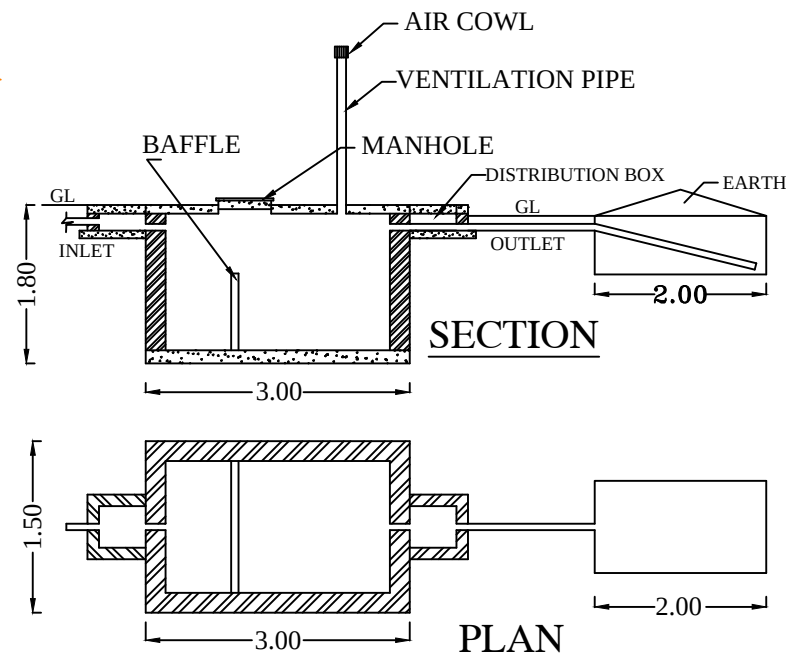
SEPTIC TANK DISPERSION TRENCH
