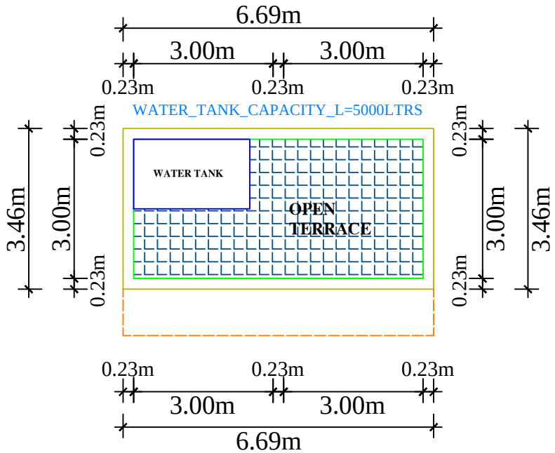
TERRACE PLAN
