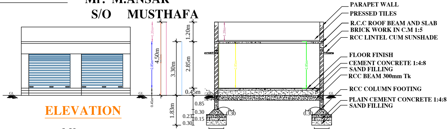
SECTION [A-A]
