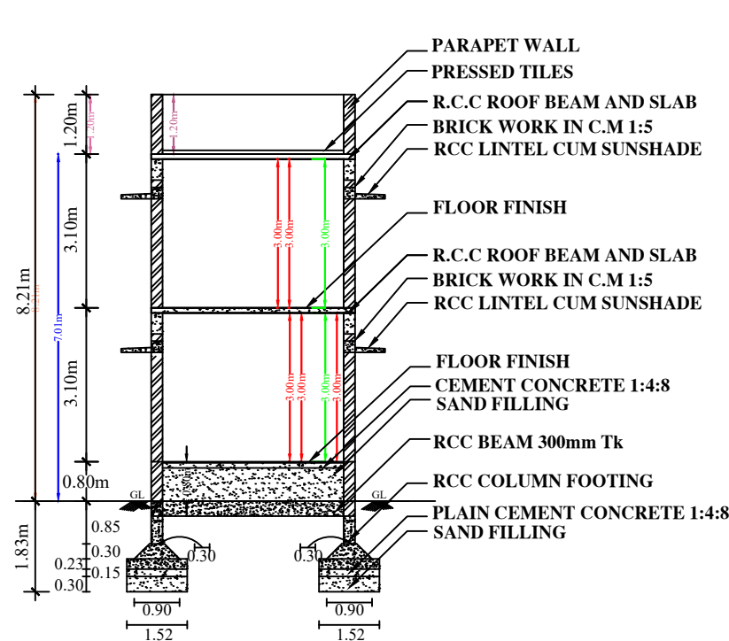
SECTION [A-A]
