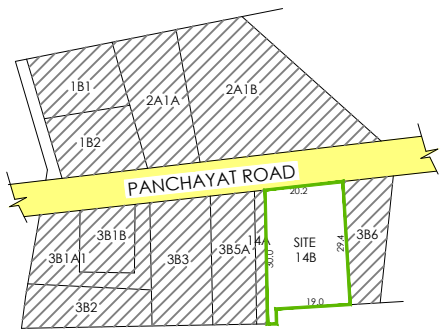
SITE PLAN SCALE:1:300
