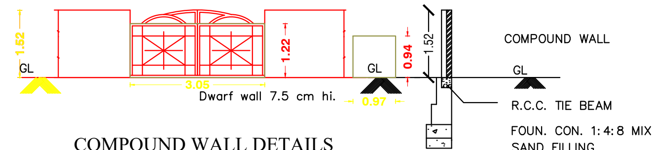
SECTION
