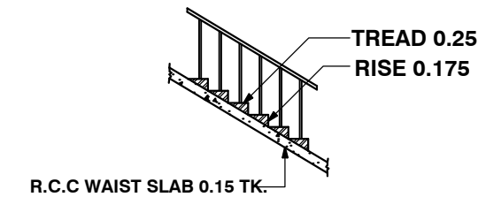
STAIR CASE DETAILS
