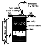
SEC. RAIN WATER HARVEST PIT
