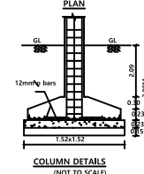
COLUMN DETAILS
