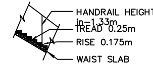
STAIRCASE DETAILS
