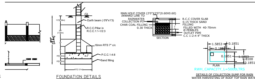
FOUNDATION DETAILS
