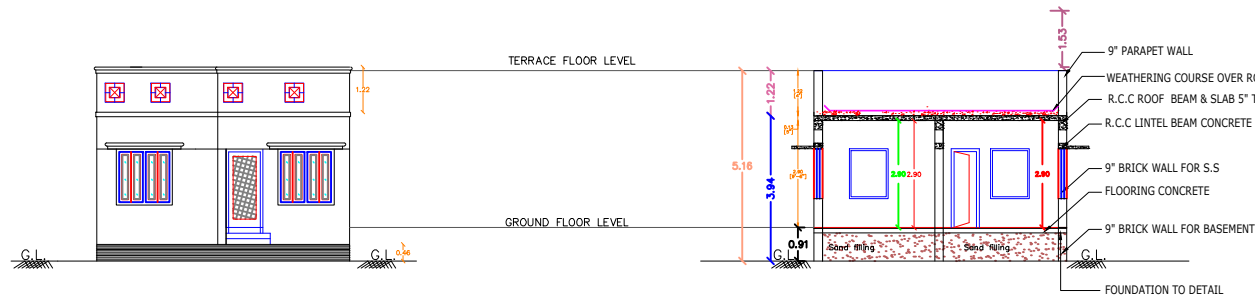
FRONT ELEVATION
