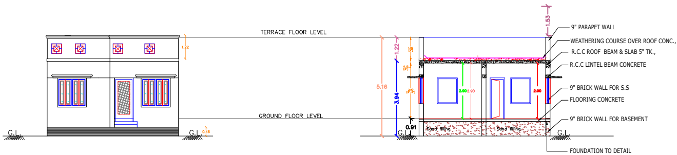
FRONT ELEVATION
