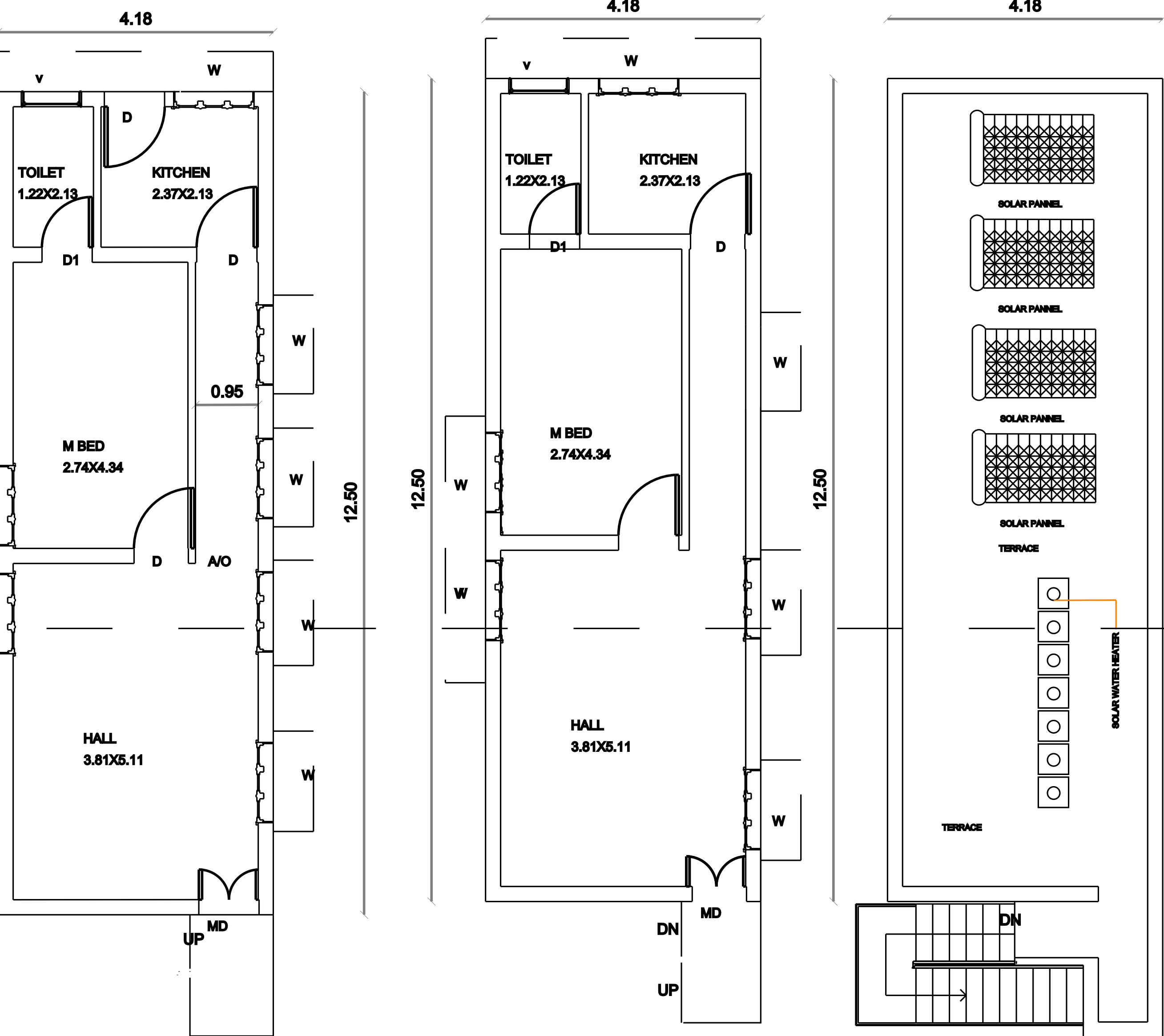
FIRST FLOOR
