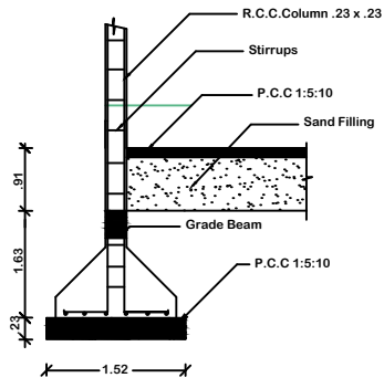
COLUMN DETAIL
