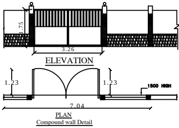
Compound wall Detail
