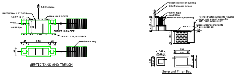
SECTION-AB
