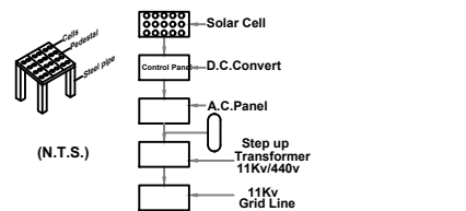
SOLAR SYSTEM FLOW DIAGRAM
