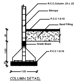
COLUMN DETAIL
