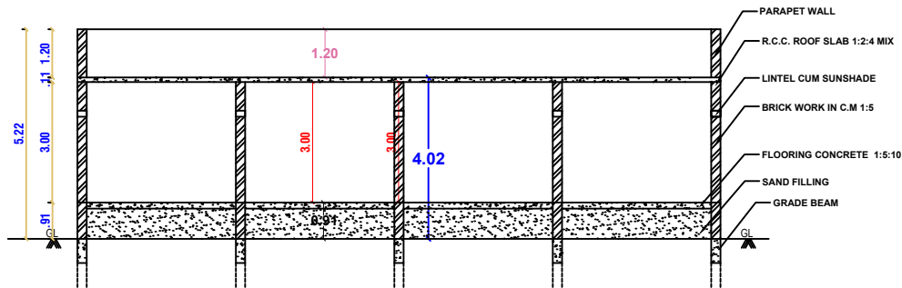
SECTION-AB
