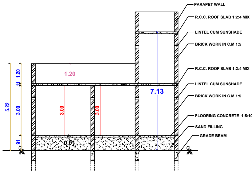
SECTION-AB
