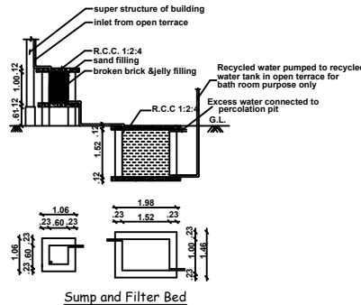
Sump and Filter Bed
