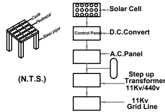
SOLAR SYSTEM FLOW DIAGRAM
