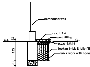
PLINTH BOUNDARY PERCOLATION PIT
