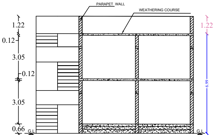
Section on-"AA"
