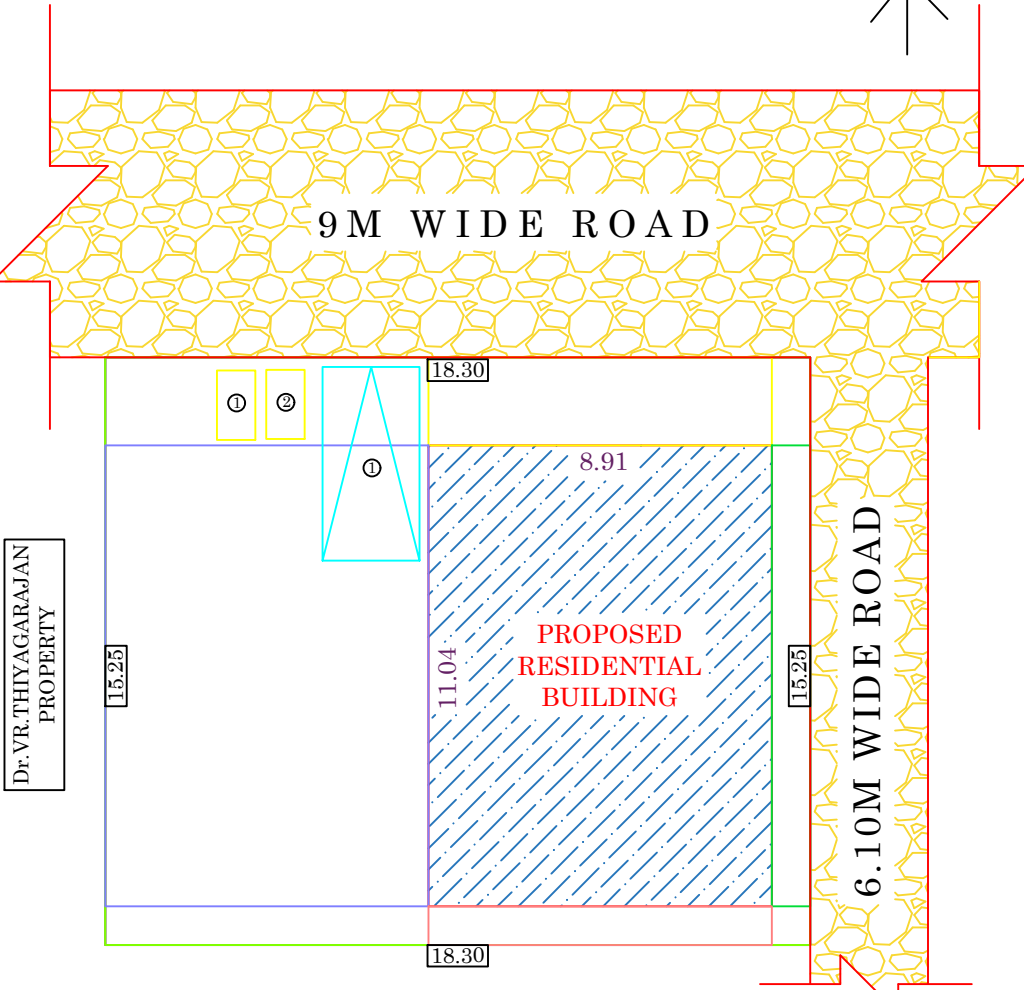
SITE PLAN
