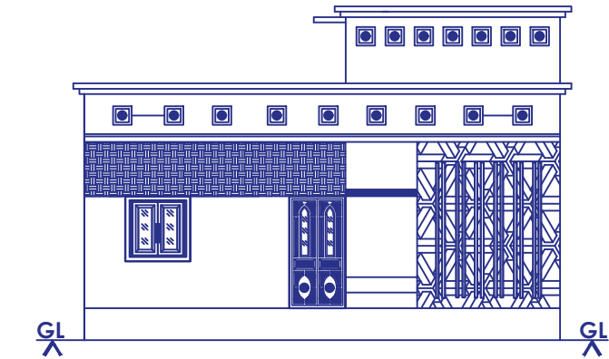
FRONT ELEVATION
