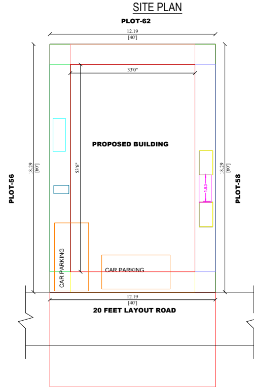
SITE PLAN
