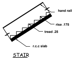
STAIR
