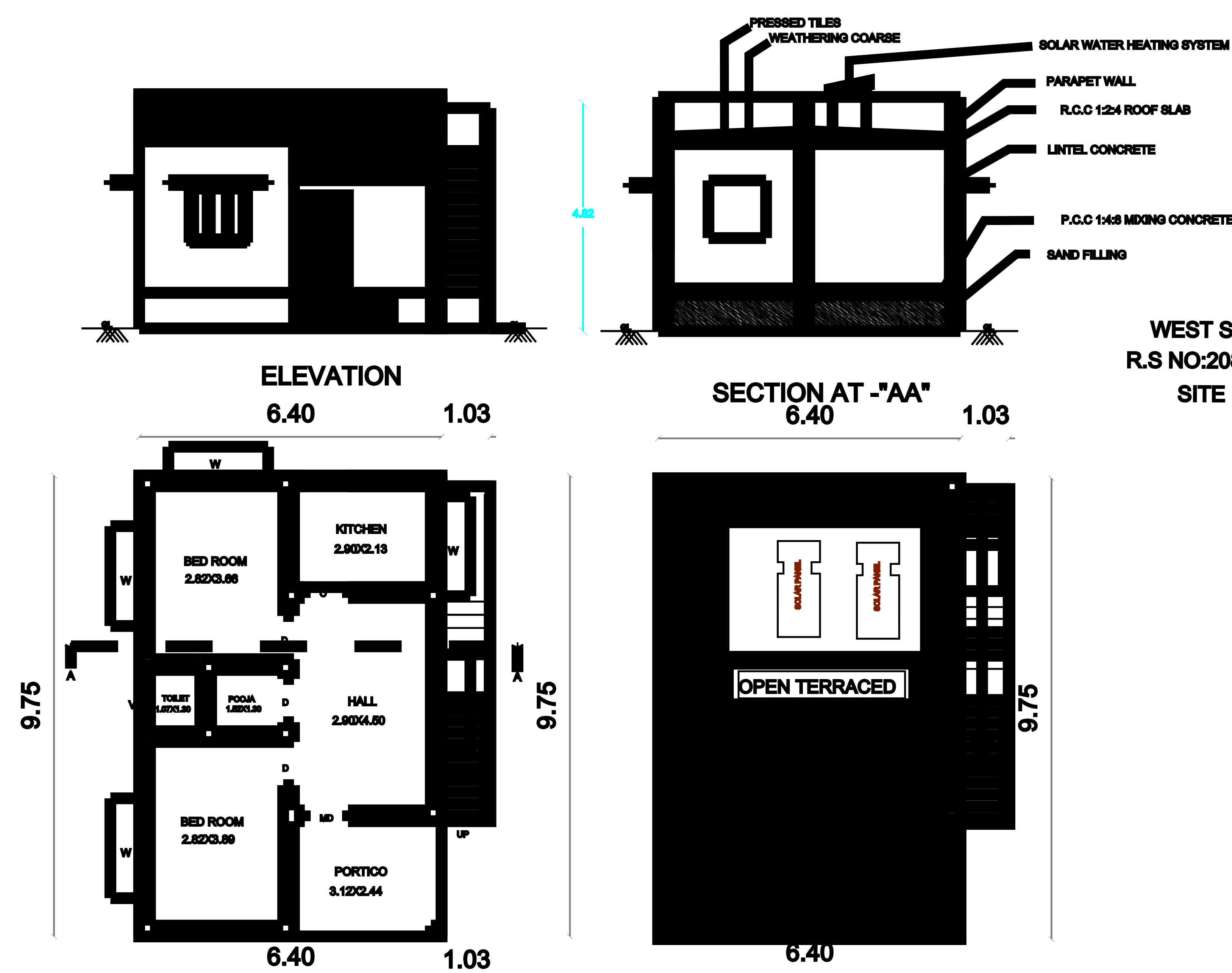
PRO.GROUND FLOOR PLAN
