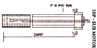
BOREWELL DETAILS
