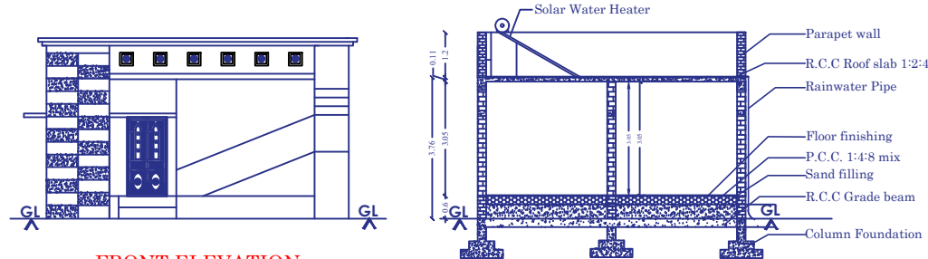
FRONT ELEVATION
