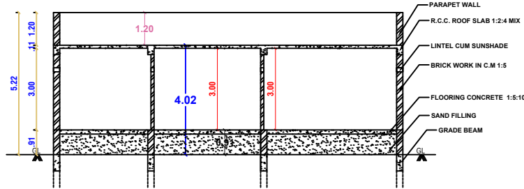
SECTION-AB
