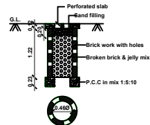
PERCOLATION PIT FOR 30 Sq. m. (Scale:- 1:50)
