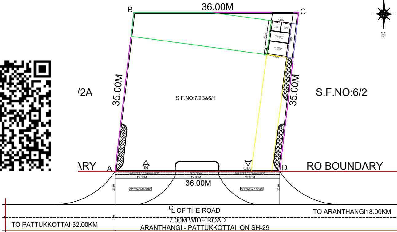
SITE PLAN
