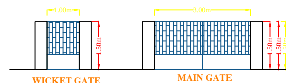
WICKET GATE
