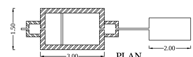
SEPTIC TANK DISPERSION TRENCH
