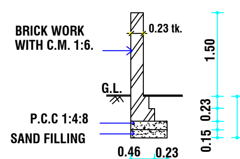
SECTION OF COMPOUND WALL
