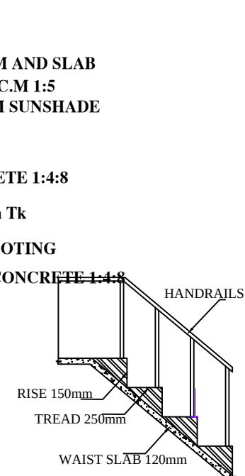
STAIRCASE DETAILS
