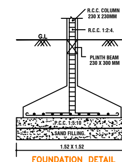
FOUNDATION DETAIL
