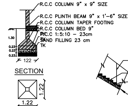
COLUMN DETAILS PLAN
