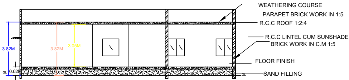
SECTION ON XX
