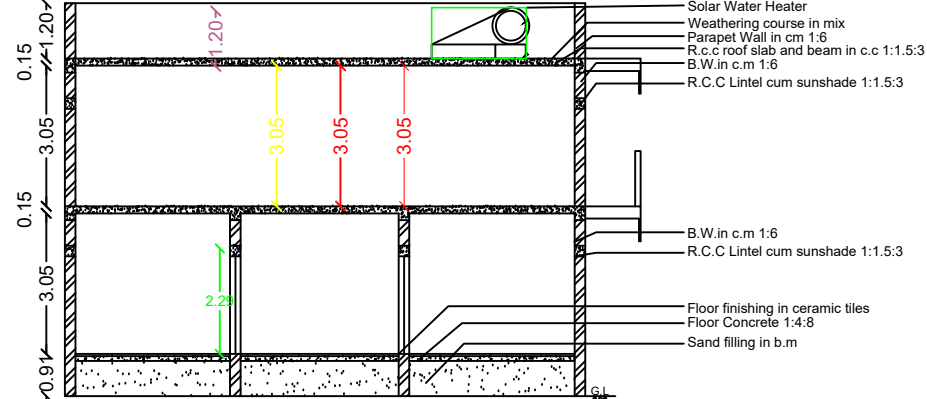
SECTION - "AB-CD"
