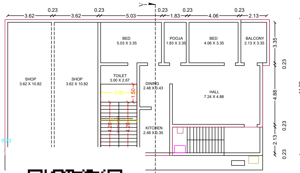
GROUND FLOOR
